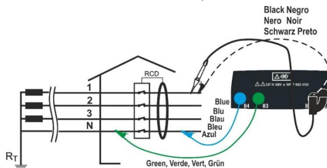
Fig. 20: Connection for a 400V + N (no PE) three-phase system by means of single cables and remote switch probe
