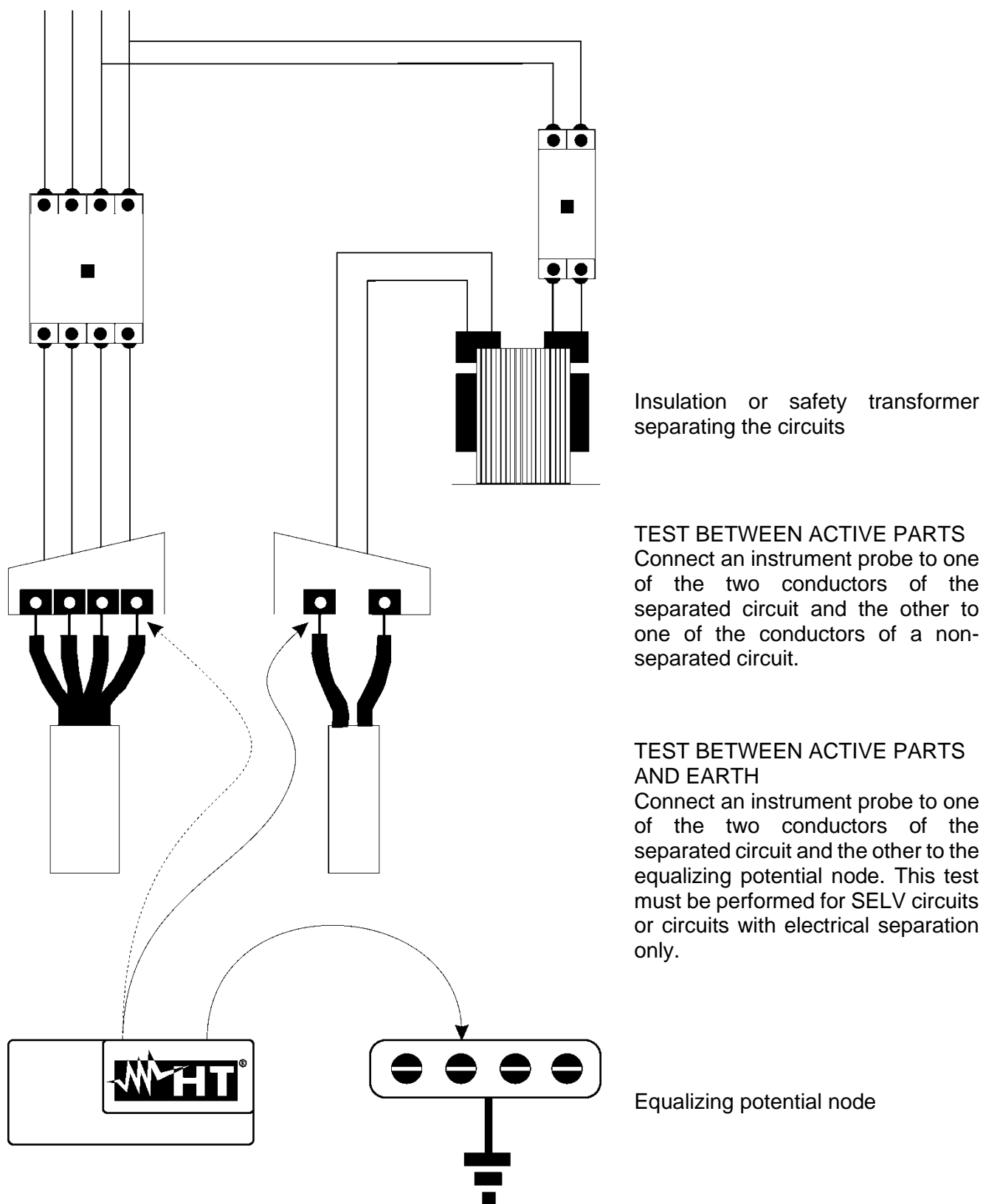
Fig. 36: Separation measurements between the circuits of a system
